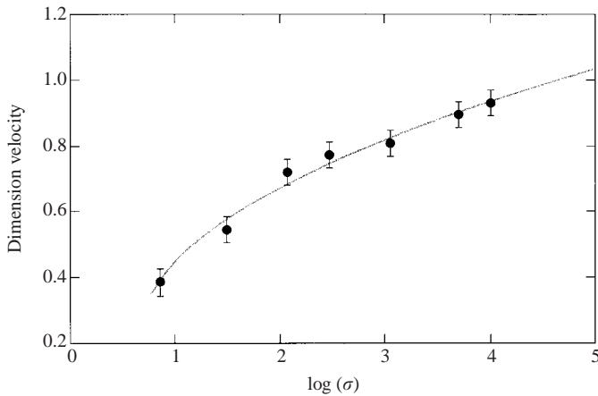
FIGURE 5. Dimensionless vertical velocity as a function of Prandtl number. ●, Present experimental results for starting plumes scaled by a factor of 1/0.57. The solid line shows the asymptotic prediction of Worster (1986) for steady plume stems.
